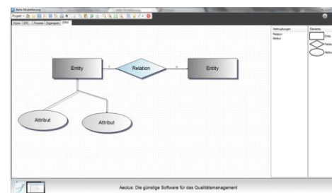
Entity-Relationship-Diagramm
